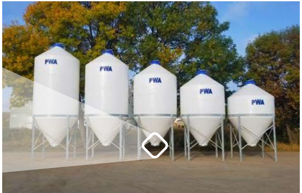
New improved lower metal auger boot transition ring on all 9'6" & 7' Diameter Polybins.
